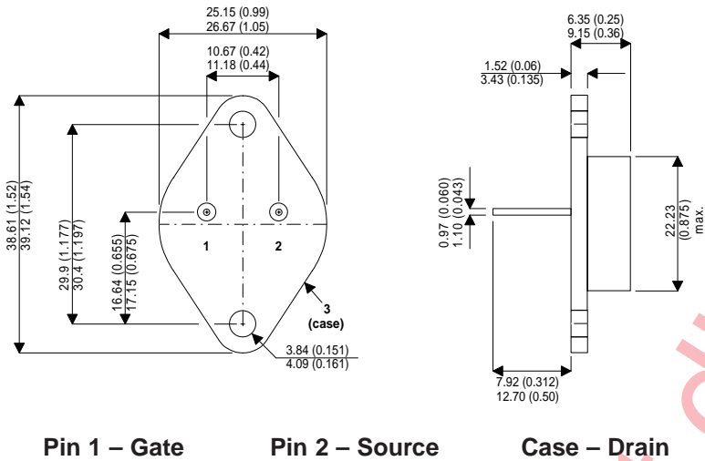
TO-3 (TO-204AA) Package Outline. Dimensions in mm (inches)
