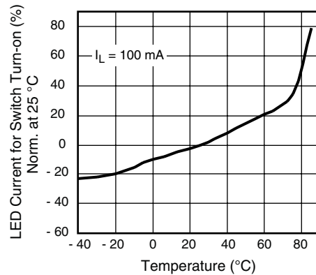
Fig. 5 - LED Current for Switch Turn-on vs. Temperature
