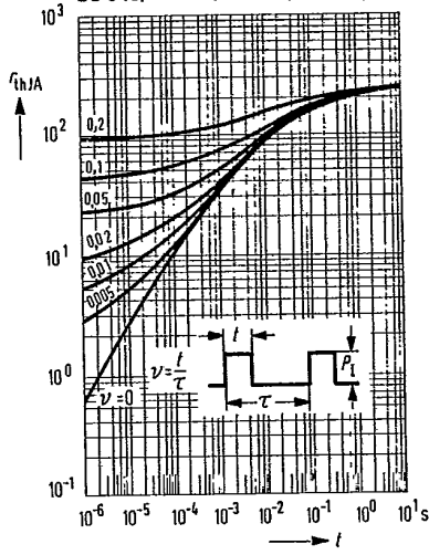
Permissible pulse load r_{thJA} = f(t) v = \text{parameter} BC 546, BC 547, BC 548, BC 549, BC 550
