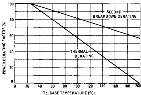
FIGURE 9 — POWER DERATING
