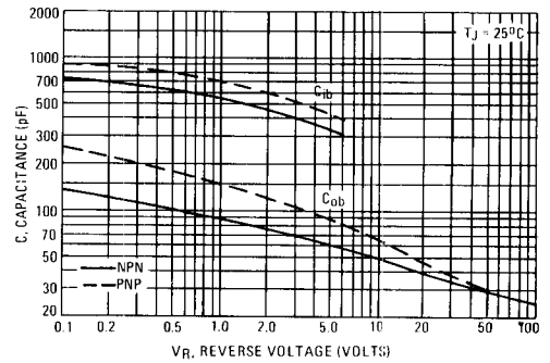
FIGURE 5 — CAPACITANCE
