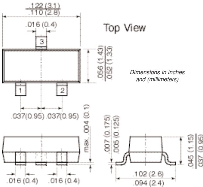
TO-236AB (SOT-23)
