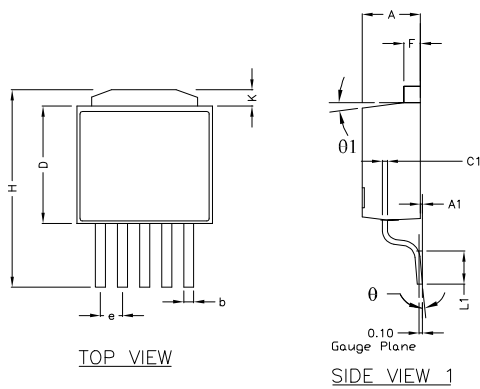
SIDE VIEW 1
