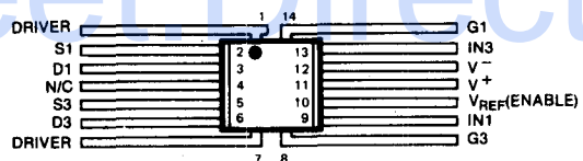
OUTLINE DWG FD-2
