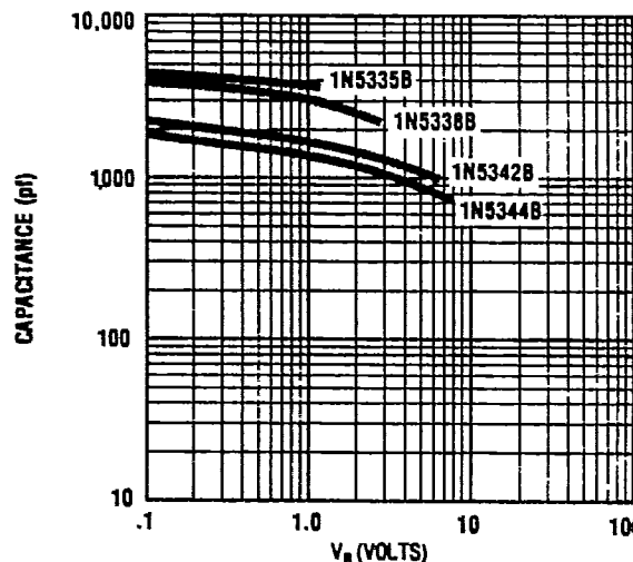
FIGURE 6 TYPICAL CAPACITANCE VS. REVERSE VOLTAGE FOR 5 WATT ZENERS
