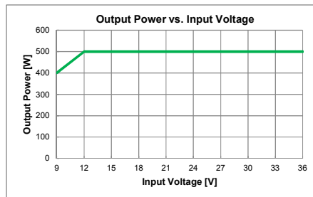
Fig. A : Output Power vs. Input Voltage
