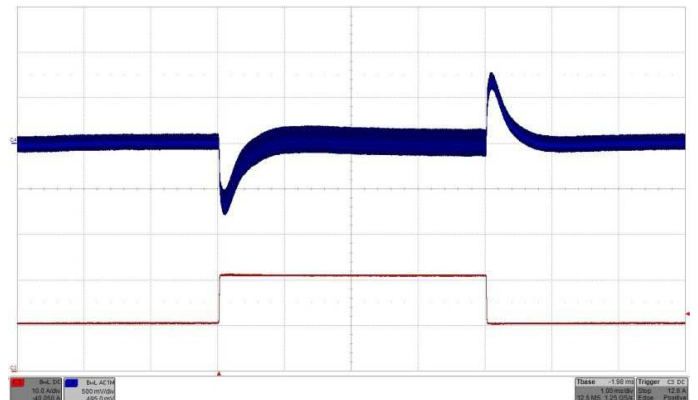
Fig. 25: Output voltage response to load current step change 100% - 50% (10.5A - 21A - 10.5A) with di/dt = 1A/\mu s at V_{IN} = 24V . Top trace (C4): Output voltage (500 mV/div.). Bottom trace (C3): Load current (10A/div.). C_O 470 \mu F /70m \Omega . Time: 1ms/div.
