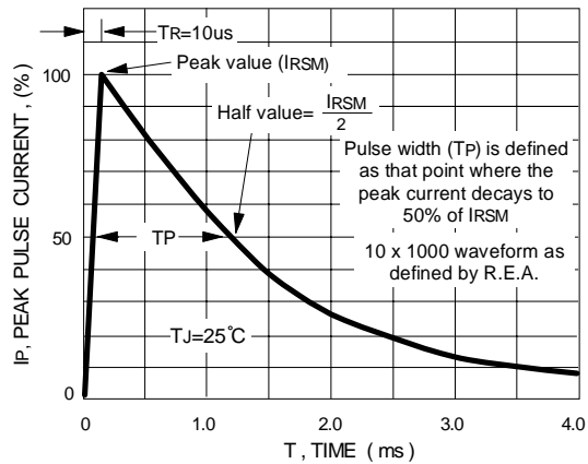
FIG.5 - PULSE WAVEFORM
