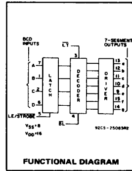
FUNCTIONAL DIAGRAM
