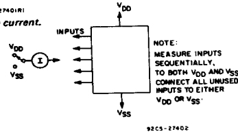
Fig. 11 - Input current.
