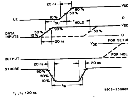
Fig. 14 - Dynamic waveforms.
