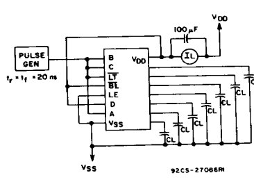
Fig. 13 - Dynamic power dissipation.
