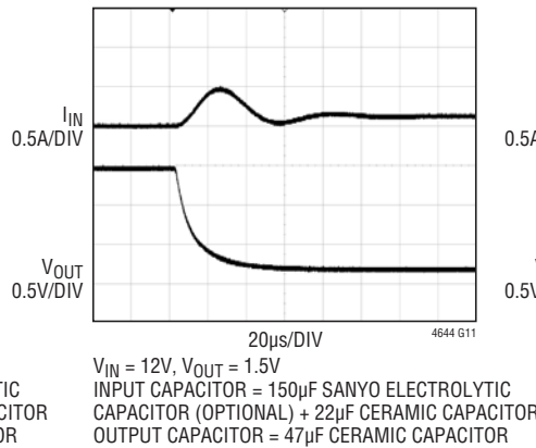
Short-Circuit with No Load
