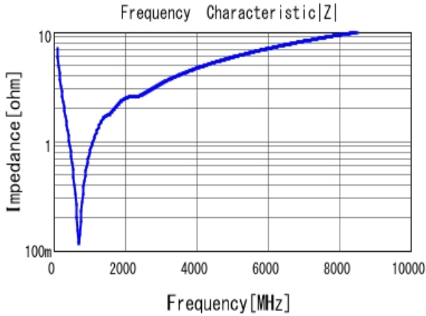
■ GRM0335C1H221JA01 |Z| DC0V, 25degC
