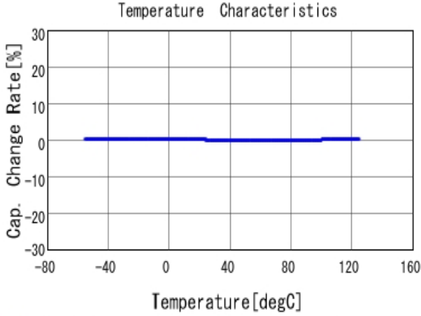
■ GRM0335C1H221JA01 C-Temp. capchange, DCOV, AC1Vrms
