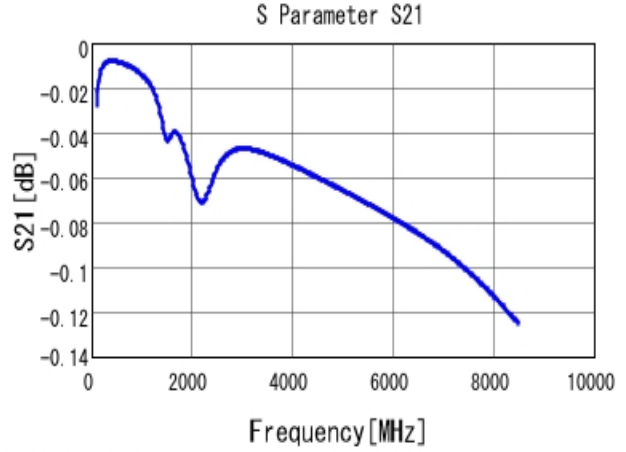
■ GRM0335C1H221JA01 S21 DCOV, 25degC
