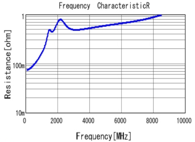
■ GRM0335C1H221JA01 R DC0V, 25degC
