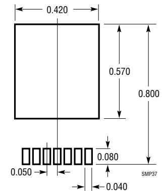
T7 Package 7-Lead TO-220 (Flow 35)
