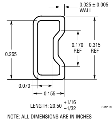
SW (0.300) SO Package Shipping Tube
