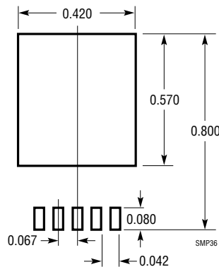
T5 Package 5-Lead TO-220 (Flow 33)
