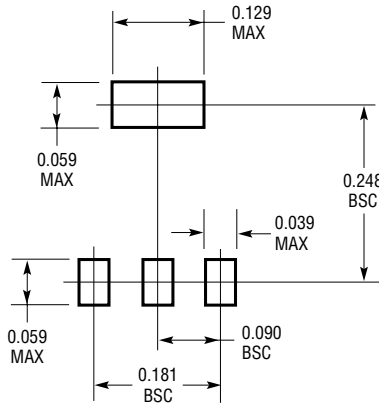
ST Package 3-Lead SOT-223
