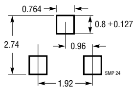
S3 Package 3-Lead SOT-23
