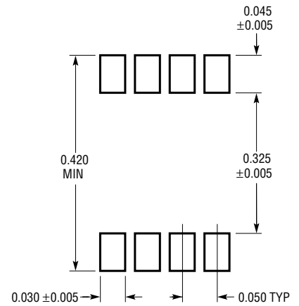
SW Package Wide (0.300) SO-16, SO-18, SO-20, SO-24, SO-28
