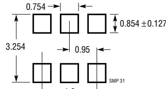
S6 Package 6-Lead SOT-23
