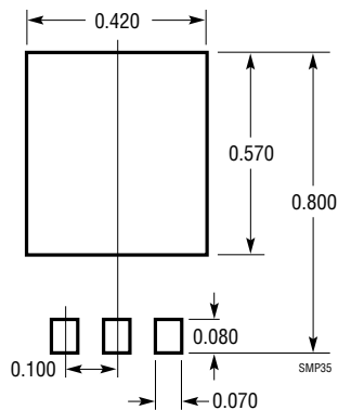
T3 Package 3-Lead TO-220 (Flow 32)
