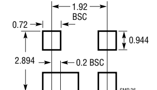
S4 Package 4-Lead SOT-143
