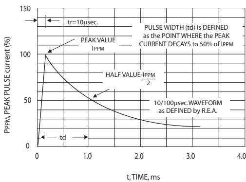
FIG.3-PULSE WAVEFORM
