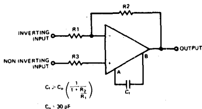
STANDARD CIRCUIT
