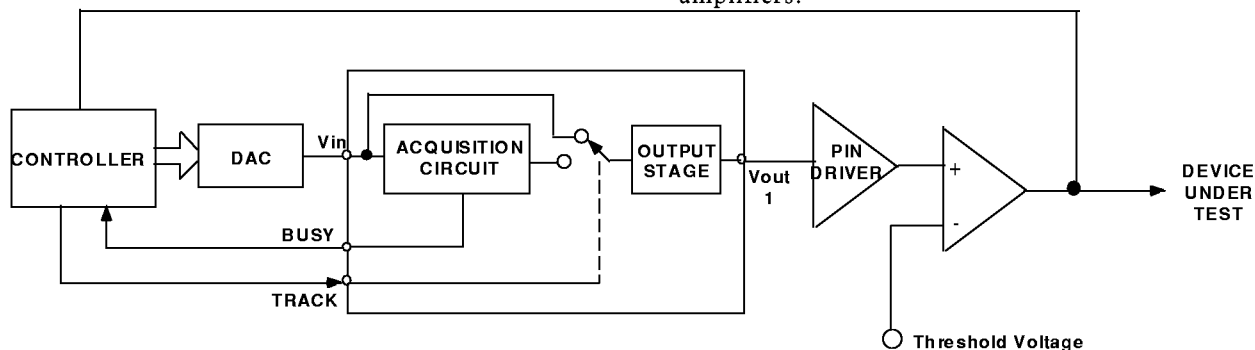
*Only one channel shown for simplicity Typical ATE circuit using TRACK Input
