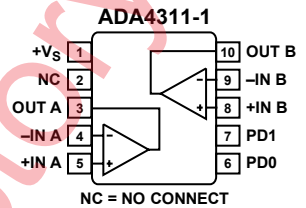
Figure 1. Thermally Enhanced, 10-Lead MINI_SO_EP
