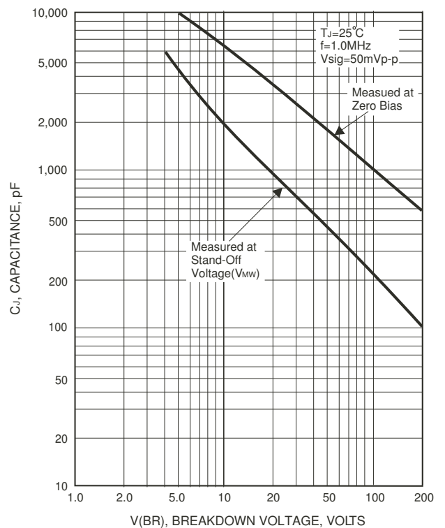
FIG.4-TYPICAL JUNCTION CAPACITANCE
