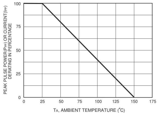
FIG.2-PULSE DERATING CURVE
