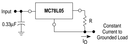
Figure 6. Current Regulator
