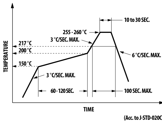
Figure 10. Recommended Pb-free reflow soldering profile
