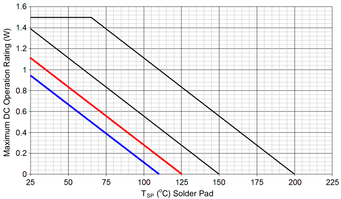
FIGURE 2 Temperature-Power Derating (R ΘJSP )
