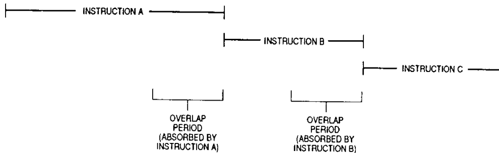
Figure 8-2. Instruction Execution for Instruction Timing Purposes
