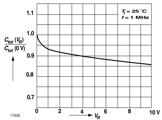
Figure 4. Relative Capacitance vs. Reverse Voltage
