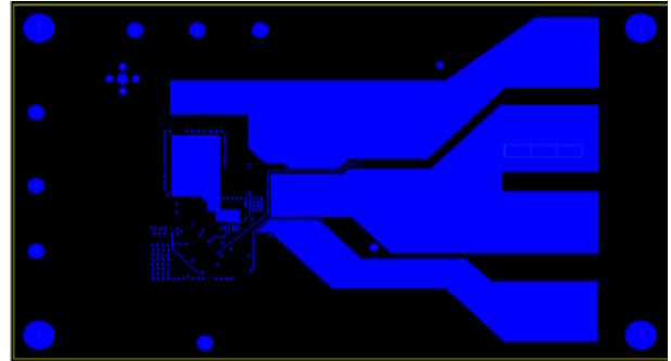
Figure 42 - Middle Layer 1
