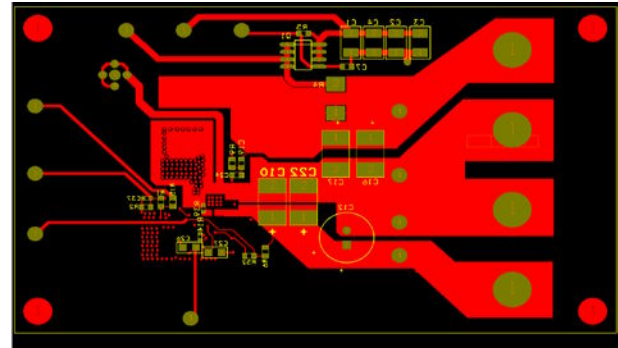
Figure 44 - Bottom Layer
