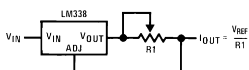
Precision Current Limiter
