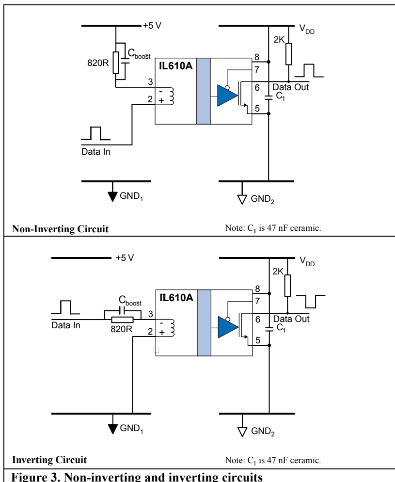
Figure 3. Non-inverting and inverting circuits
