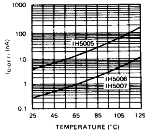
I_D(OFF) vs TEMPERATURE
