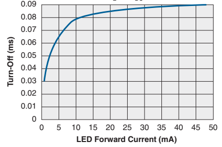
Typical Turn-Off vs. LED Forward Current ( I_L=1\text{A}_{DC} )
