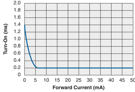
Typical Turn-On vs. LED Forward Current ( I_L=1\text{A}_{DC} )
