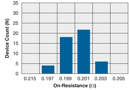
Typical On-Resistance Distribution (N=50, I_F=10\text{mA} , I_L=1\text{A}_{DC} , T_A=25^\circ\text{C} )
