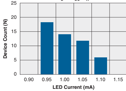
Typical I_F for Switch Operation (N=50, I_L=1\text{A}_{DC} , T_A=25^\circ\text{C} )
