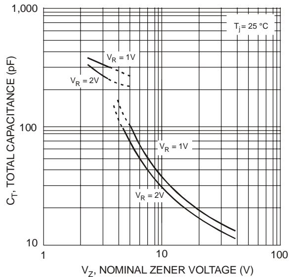
Fig. 4 Total Capacitance vs. Nominal Zener Voltage
