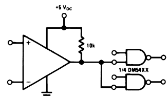
Driving TTL
