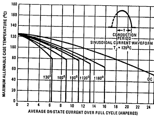
Fig. 1 - Maximum Allowable Case Temperature Vs. Average On-State Current, 2N681 Series
