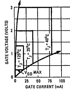
Fig. 16a — Area of All Possible Triggering Points Vs. Temperature, 2N5204 Series
