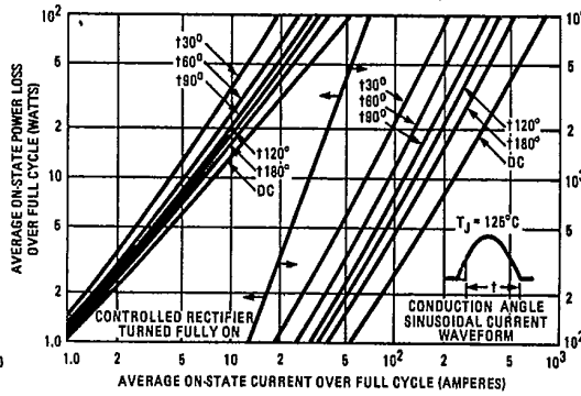
Fig. 11 - Maximum High-Level On-State Power Loss Vs. Average On-State Current (Sinusoidal Current Waveform), 2N5204 Series
