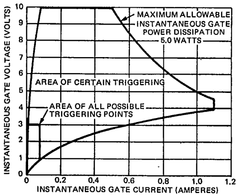
Fig. 5 - Gate Characteristics, 2N681 Series
