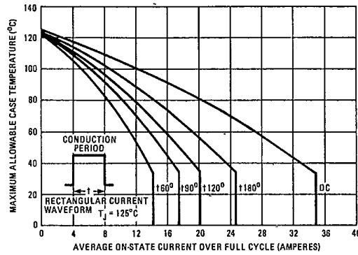
Fig. 9 - Maximum Allowable Case Temperature Vs. Average On-State Current (Rectangular Current Waveform), 2N5204 Series
