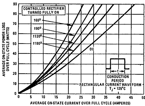
Fig. 12 - Maximum Low-Level On-State Power Loss Vs. Average On-State Current (Rectangular Current Waveform), 2N5204 Series
