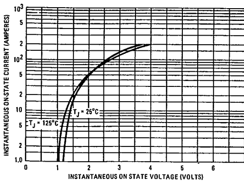
Fig. 14 - Maximum Instantaneous On-State Voltage Vs. Instantaneous On-State Current, 2N5204 Series
