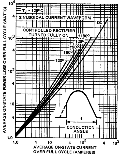
Fig. 4 - Maximum High Level On-State Power Loss Vs. Current (Sinusoidal Current Waveform), 2N681 Series
