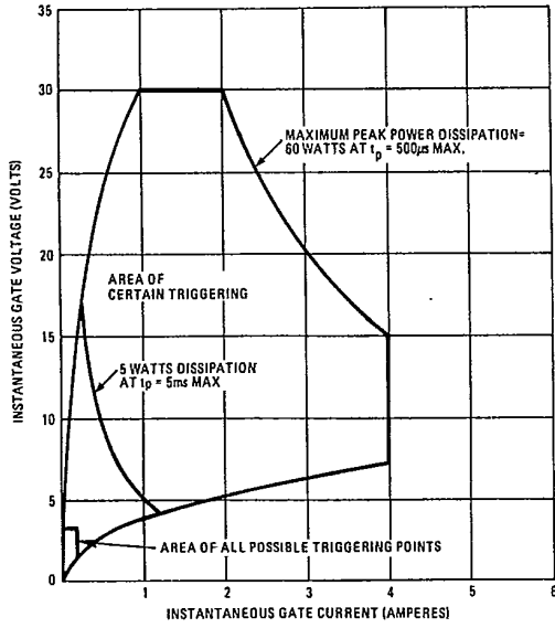
Fig. 16 — Gate Characteristics, 2N5204 Series
