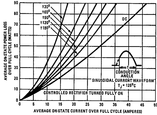
Fig. 10 - Maximum Low-Level On-State Power Loss Vs. Average On-State Current (Sinusoidal Current Waveform), 2N5204 Series
