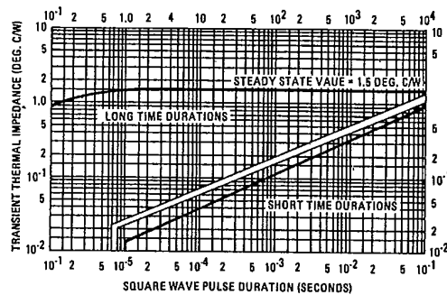
Fig. 15 - Maximum Transient Thermal Resistance, Junction to Case, Vs. Pulse Duration, 2N5204 Series
