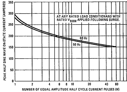
Fig. 17 — Maximum Non-Repative Surge Current Vs. Number of Current Pulses, 2N5204 Series
