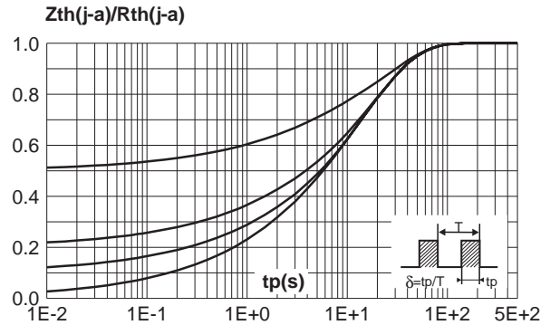
Fig. 4-2: Relative variation of thermal impedance junction to ambient versus pulse duration (epoxy printed circuit board, e(\text{Cu})=35\mu\text{m} , recommended pad layout) (SMA).
