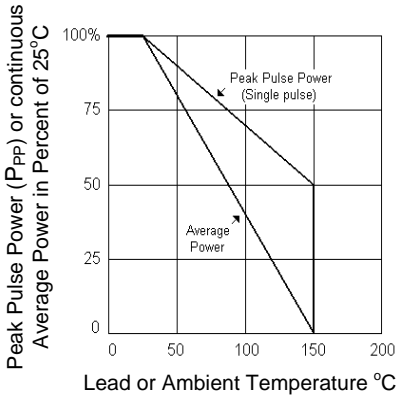
FIGURE 3 Derating Curve
