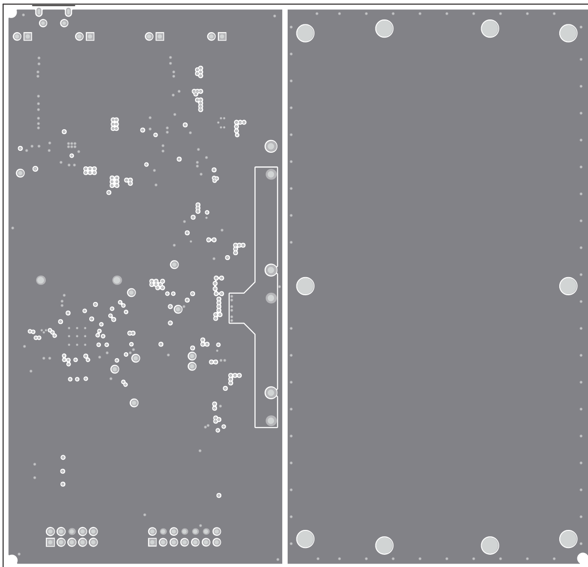
Figure 8. Layer 2
