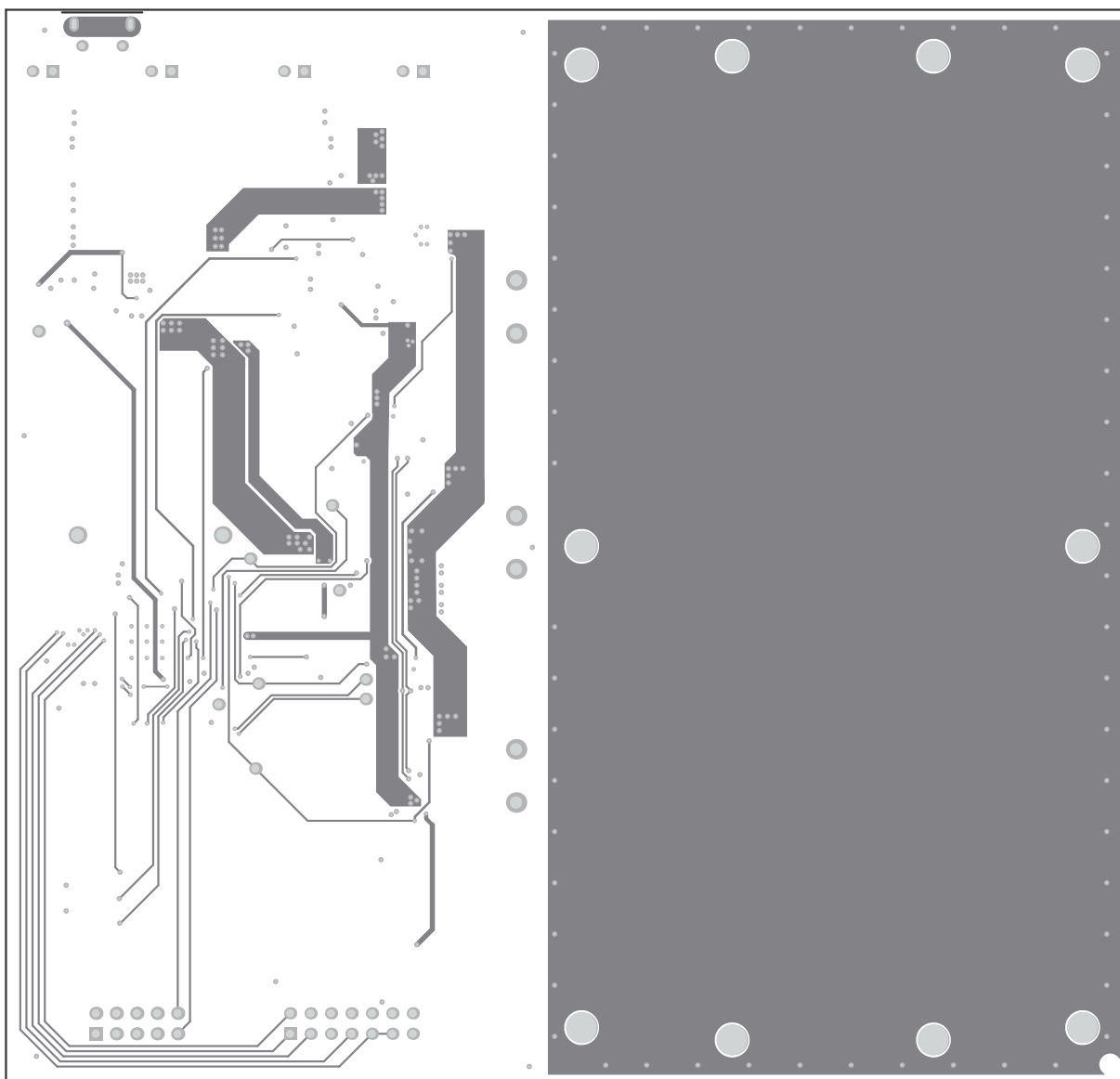
Figure 9. Layer 3
