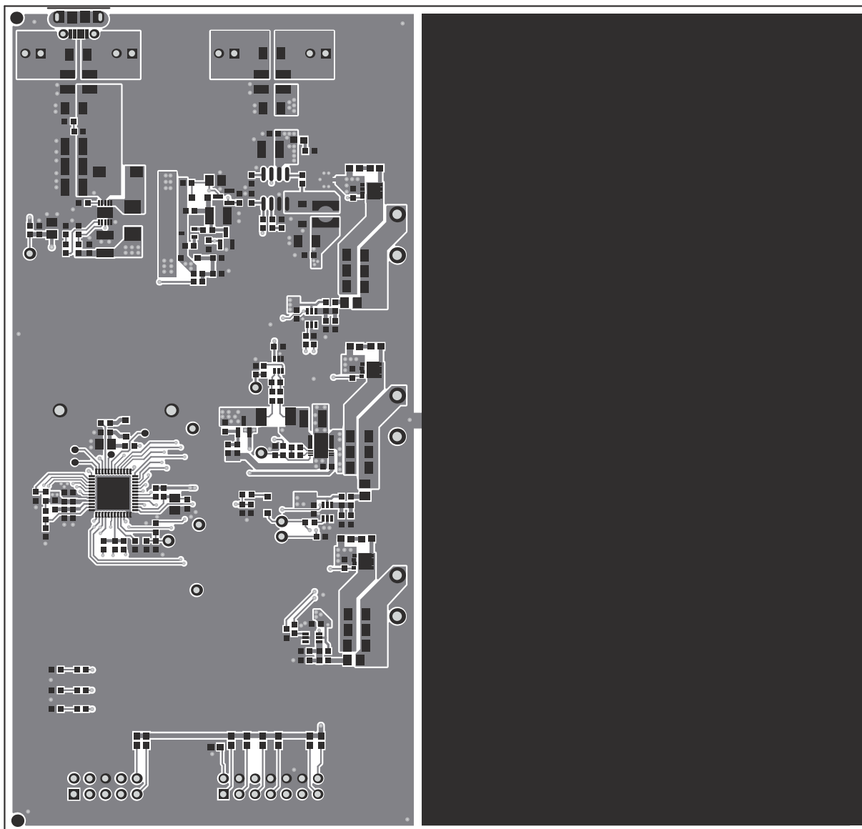
Figure 6. Top Silk
