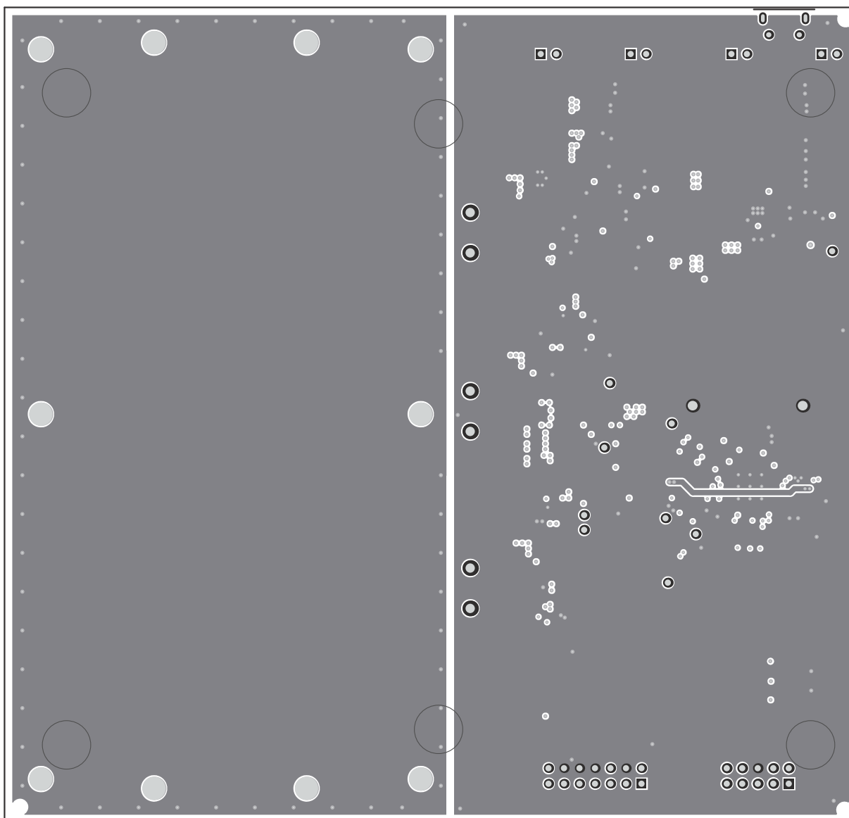
Figure 10. Bottom Layer
