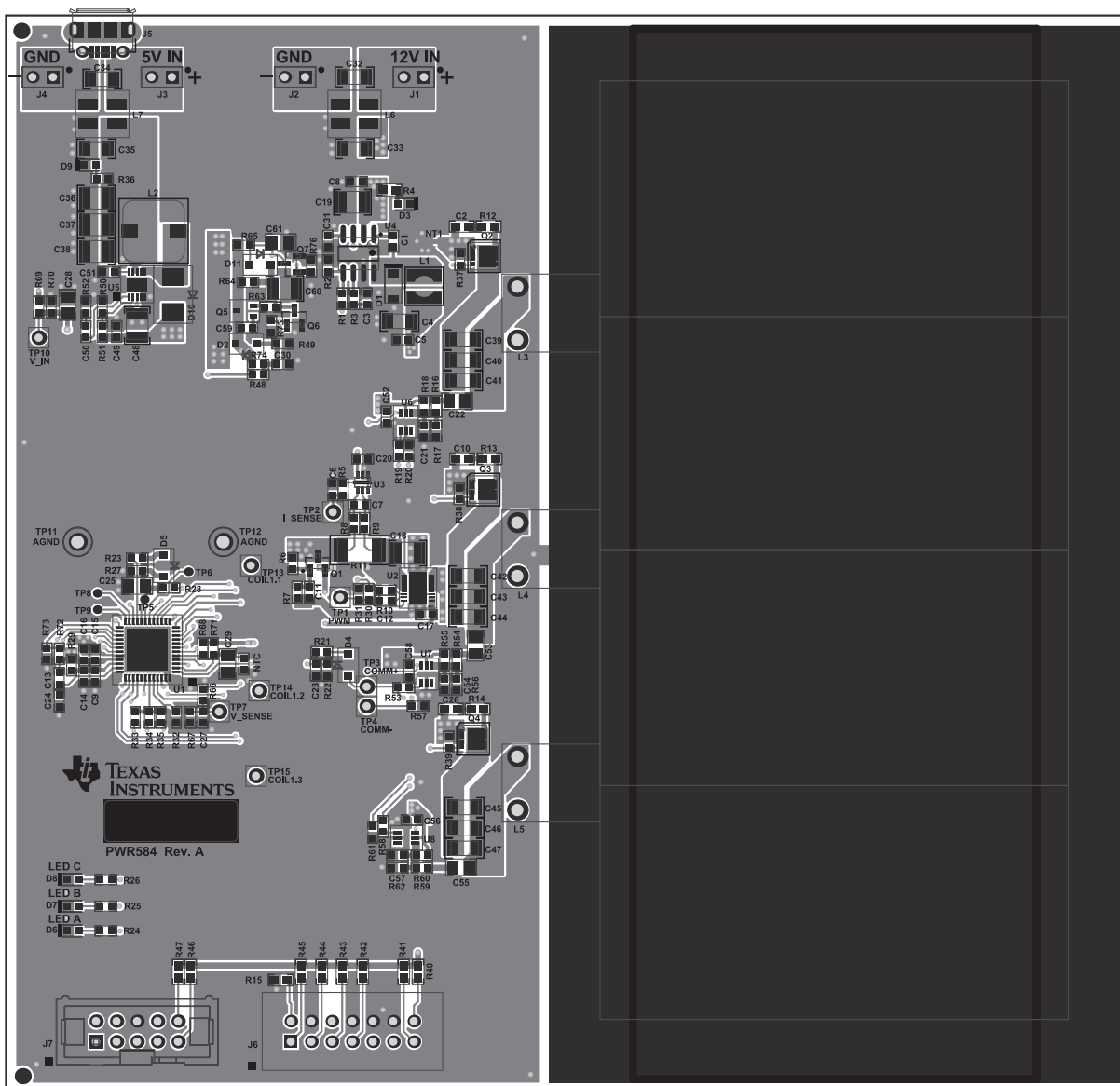
Figure 7. Top Layer
