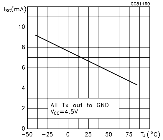
Low Level Transmitter Output Short Circuit Current vs Temperature
