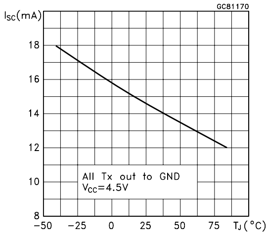
High Level Transmitter Output Short Circuit Current vs Temperature
