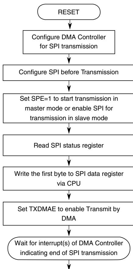
Figure 37-22. Recommended startup of SPI transmit by DMA
