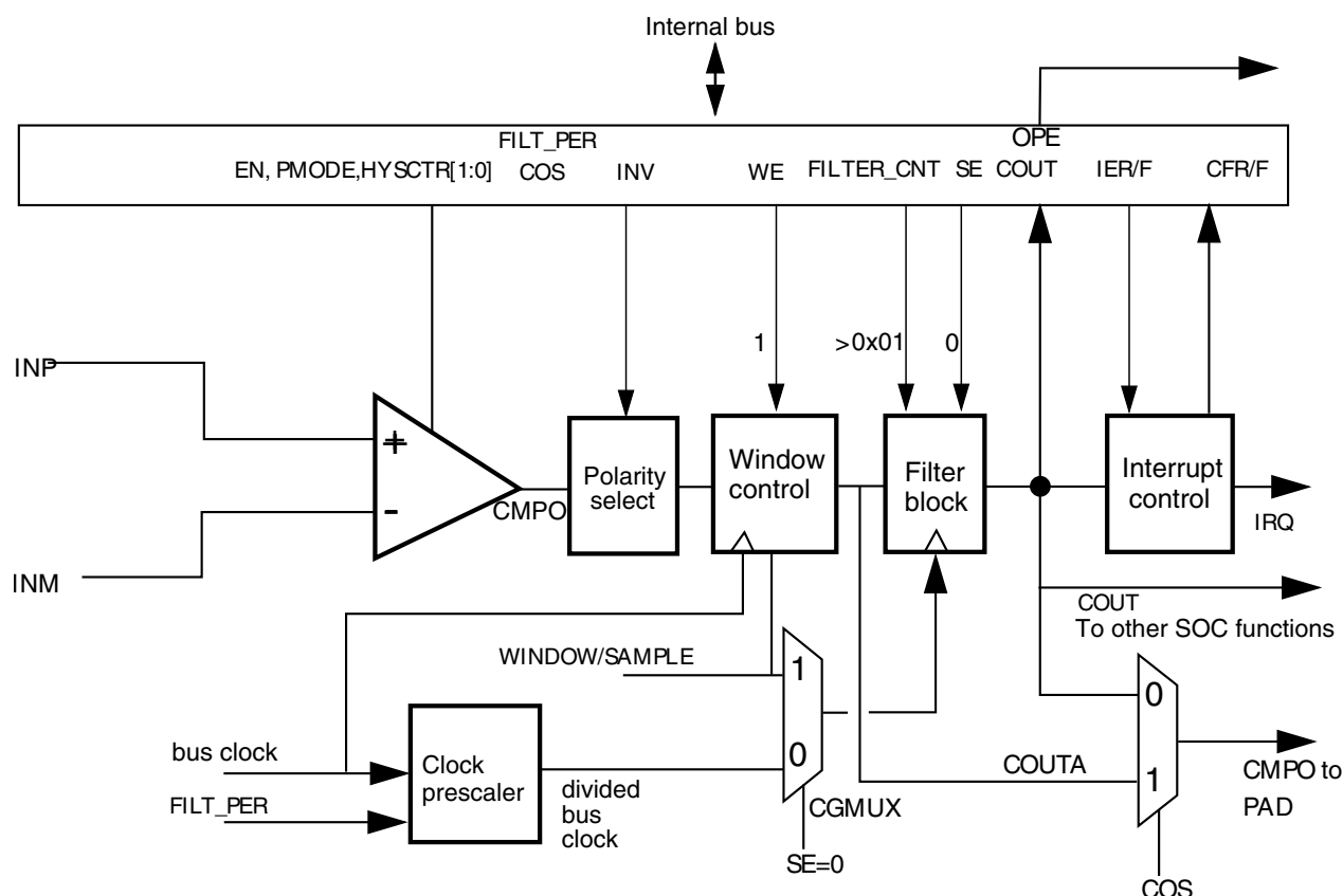
Figure 29-23. Windowed/Filtered mode
