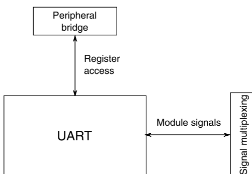
Figure 3-36. UART configuration
