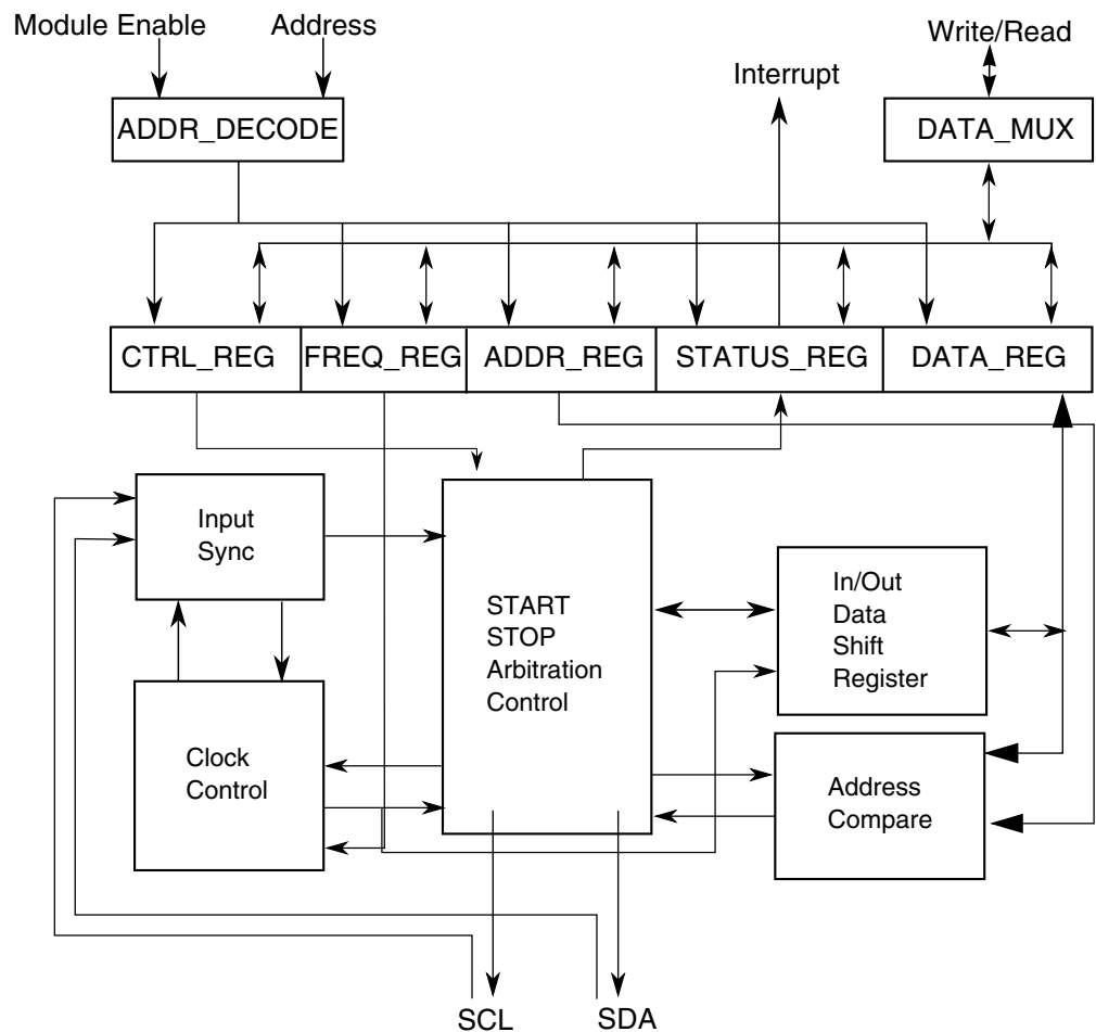
Figure 38-1. I2C Functional block diagram
