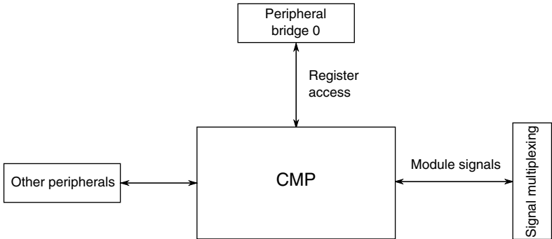
Figure 3-22. CMP configuration
