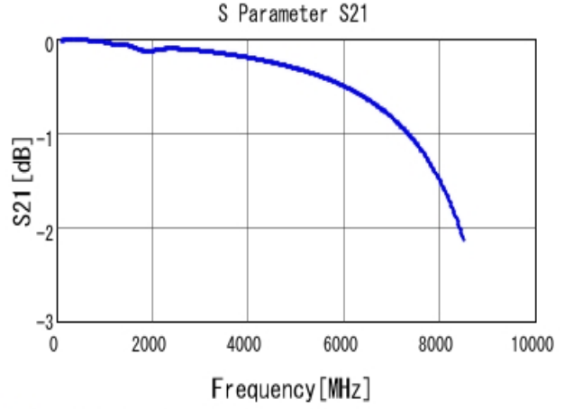
■ GCM1885C1H221JA16 S21 DCOV, 25degC
