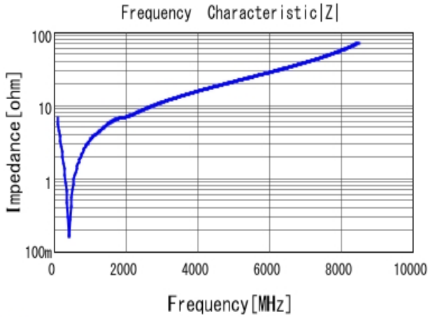
■ GCM1885C1H221JA16 |Z| DC0V, 25degC
