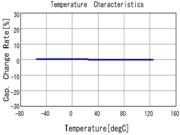
■ GCM1885C1H221JA16 C-Temp. capchange, DCOV, AC1Vrms
