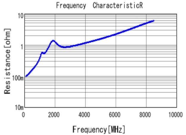
■ GCM1885C1H221JA16 R DC0V, 25degC
