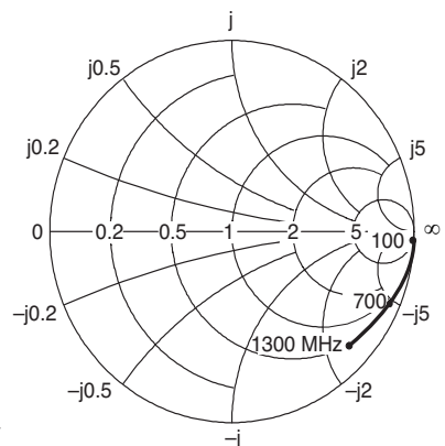
Figure 17. Output Reflection Coefficient
