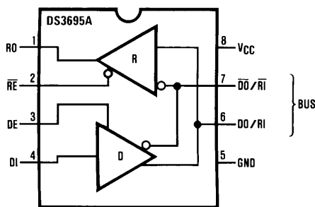
Figure 1. Molded Package, Small Outline (D0008A) Top View
