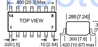
Type A1410AG (10-tap, 14-pin SM)
