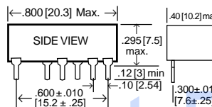
Type A1405 (5-tap, 14-pin DIP)
