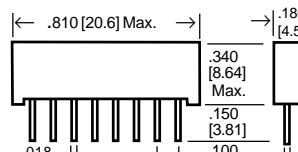
Type SA0805 (5-tap, 8-pin SIP)
