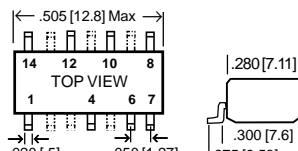
Type SMA1405 (5-tap, 14-pin SO)
