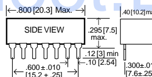
Type A1410 (10-tap, 14-pin DIP)
