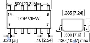
Type A1405AG (5-tap, 14-pin SM)
