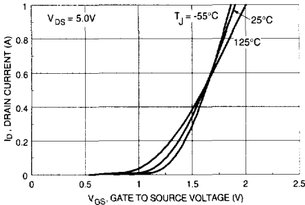
Figure 5. Transfer Characteristics.
