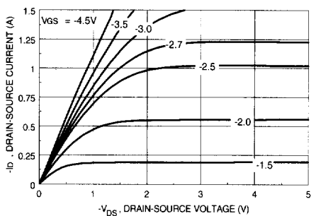
Figure 11. On-Region Characteristics.
