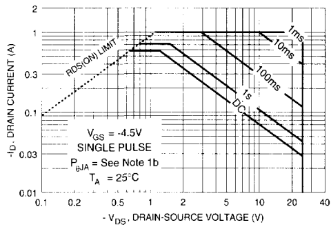
Figure 19. Maximum Safe Operating Area.
