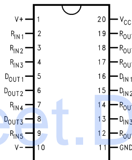
Figure 1. SOIC See Package DW0020B
