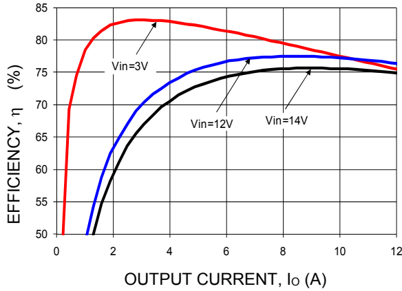
Fig-45. Converter Efficiency versus Output Current.
