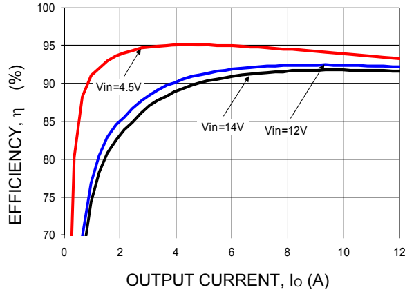
Fig-27. Converter Efficiency versus Output Current.
