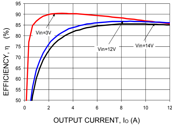
Fig-39. Converter Efficiency versus Output Current.
