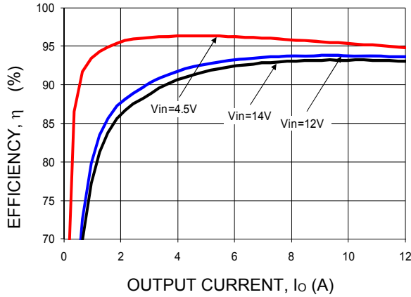
Fig-21. Converter Efficiency versus Output Current.
