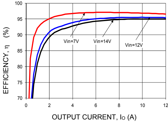
Fig-15. Converter Efficiency versus Output Current.
