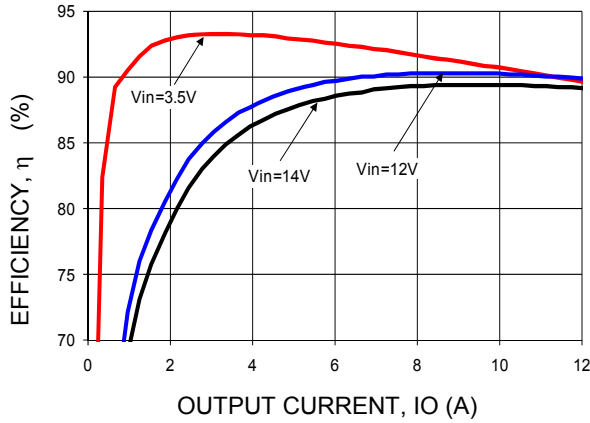
Fig-33. Converter Efficiency versus Output Current.
