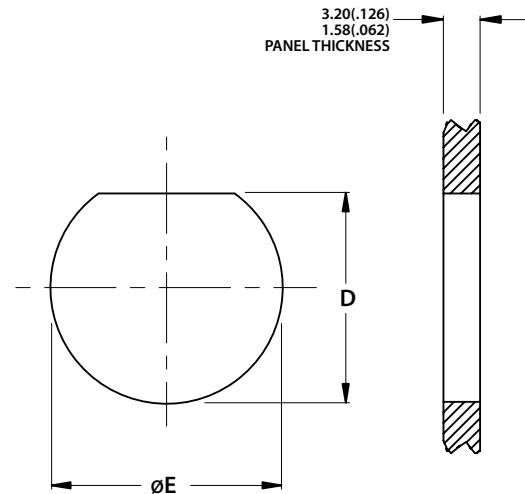
JAM NUT MOUNT
