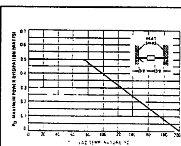
Figure 2 POWER DERATING CURVE
