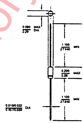
FIGURE 1 all dimensions in INCH mm
