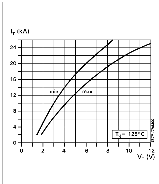
Fig. 3 On-state characteristics, T_{vj} = 125\text{ }^{\circ}\text{C} , 10 ms half sine
