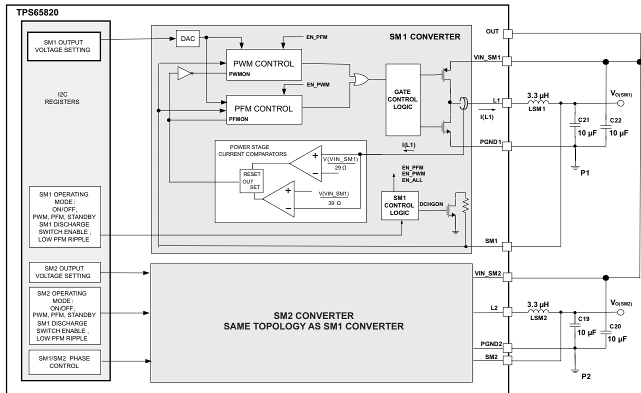
Figure 42. SM1/SM2 Converter
