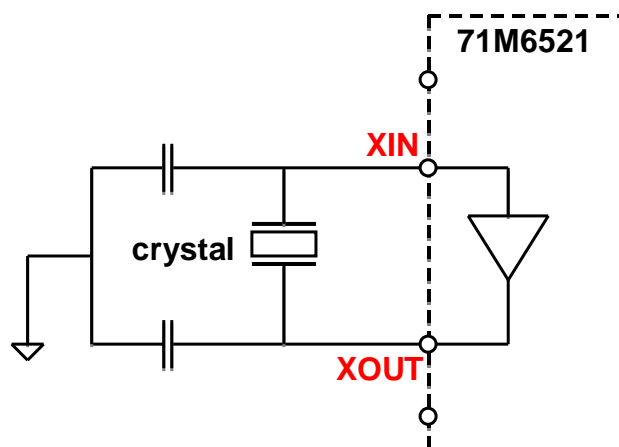
Figure 2-9: Oscillator Circuit
