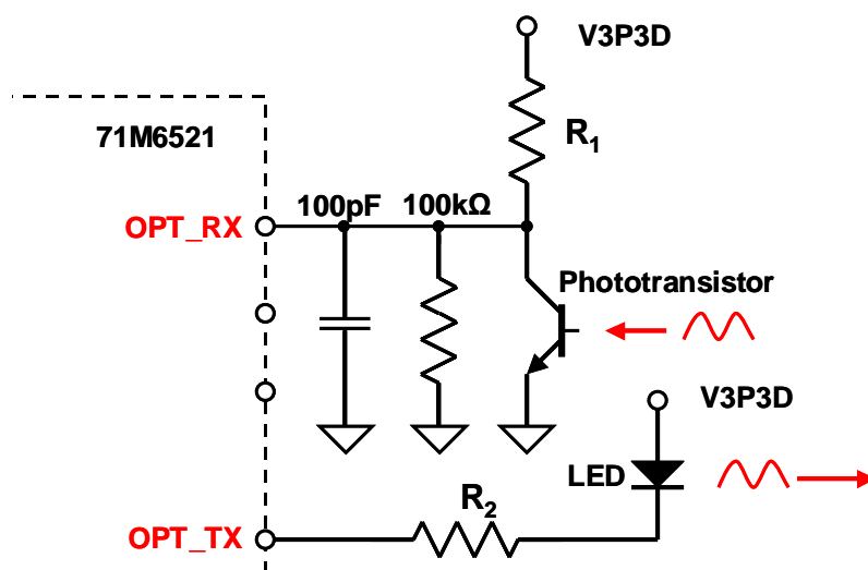
Figure 2-13: Optical Interface Block Diagram
