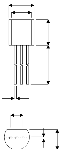
TO92 PACKAGE
